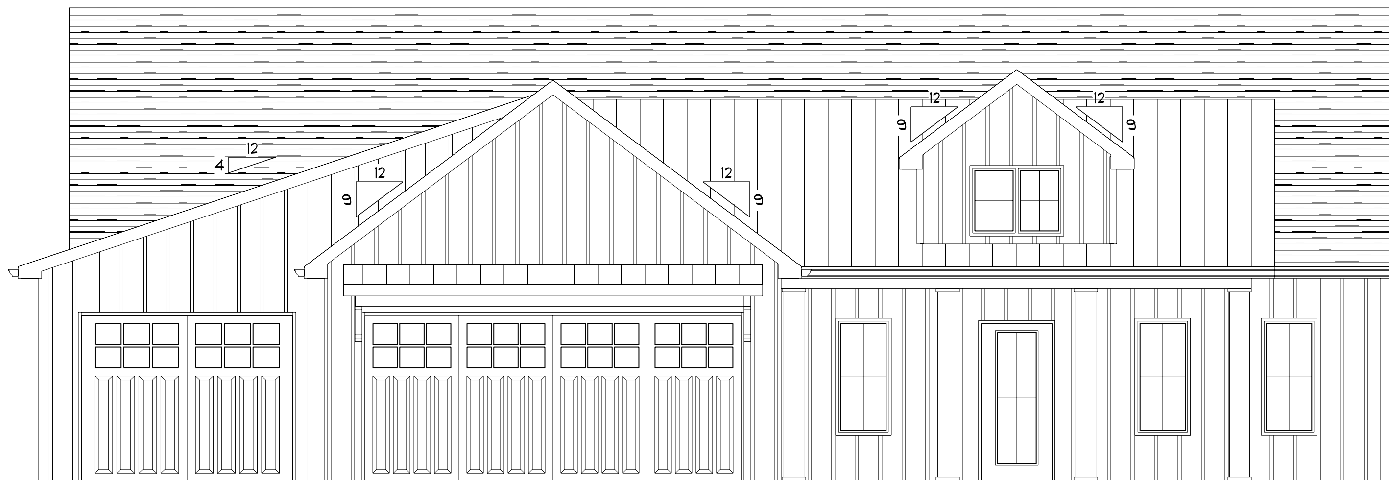
FRONT ELEVATION
