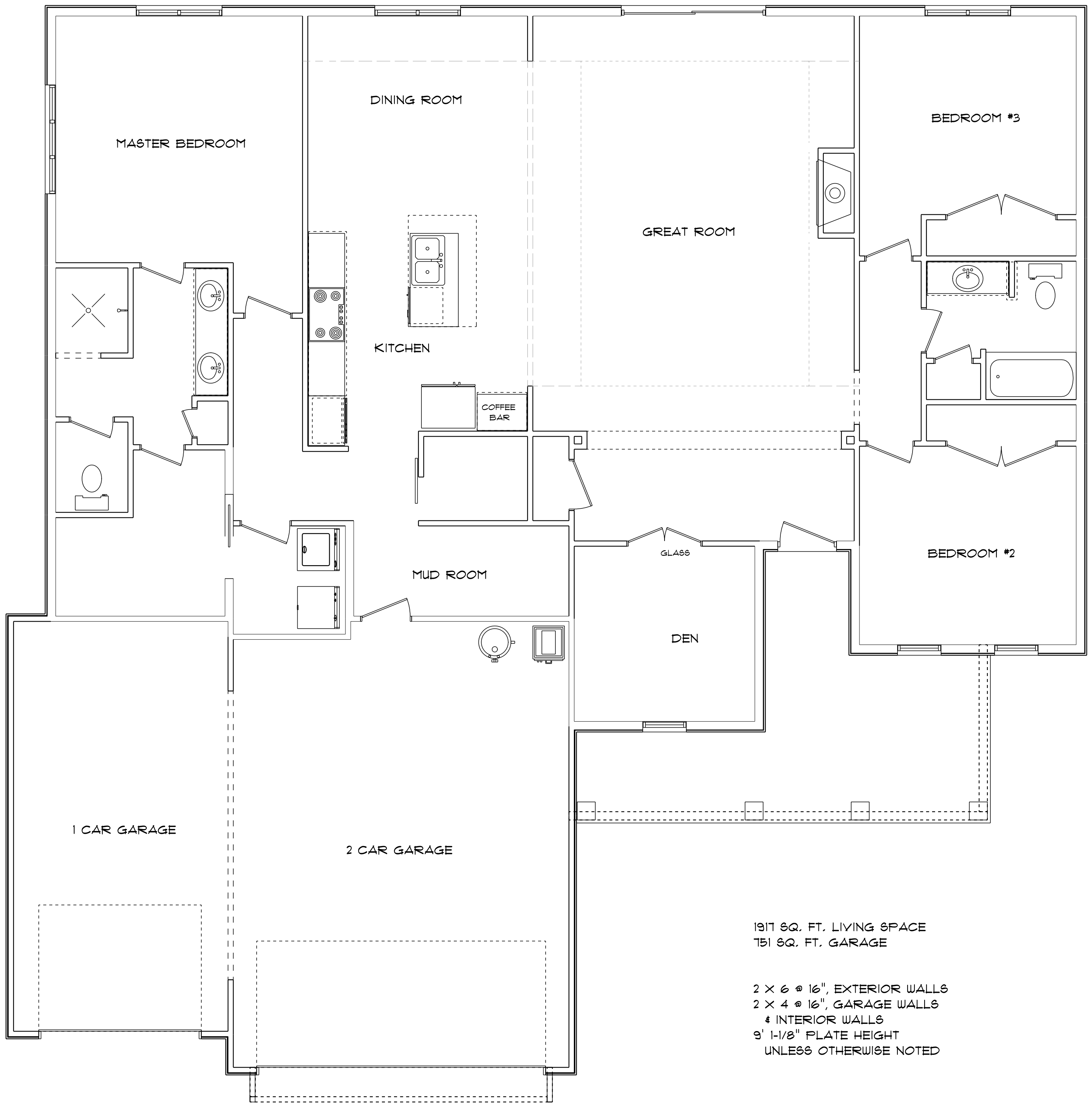
1ST FLOOR LAYOUT
